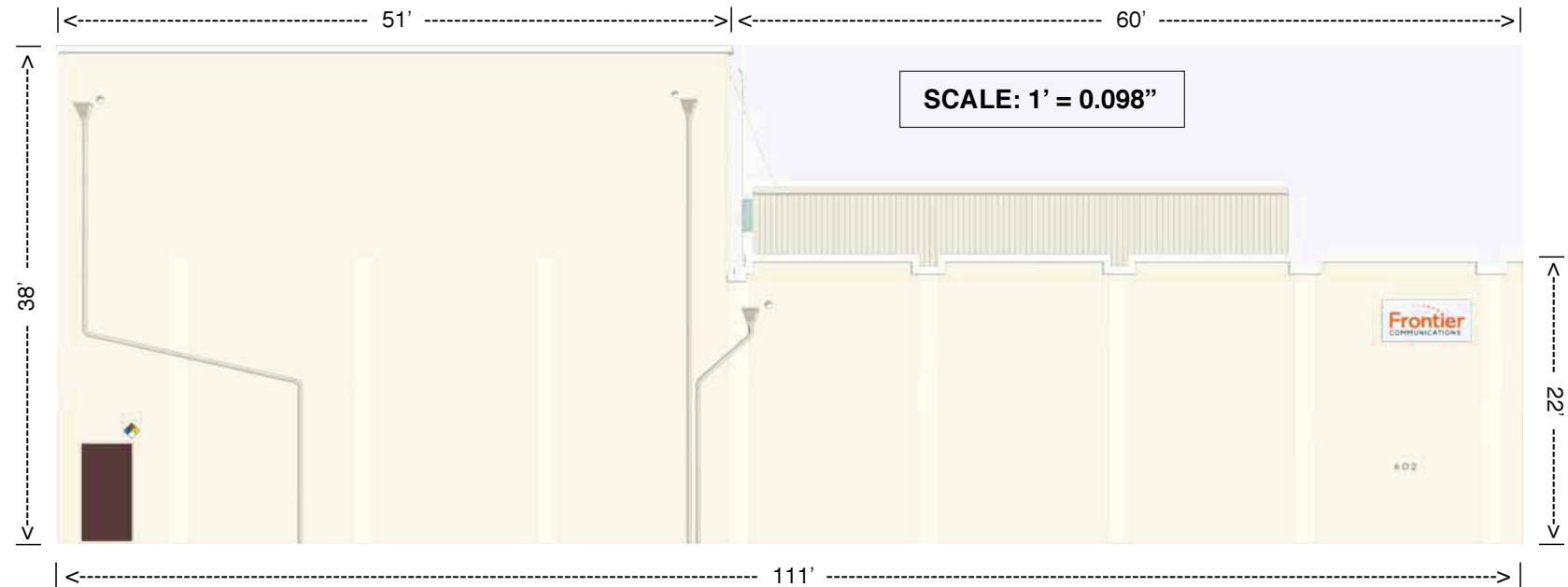
MAIN STREET ELEVATION
