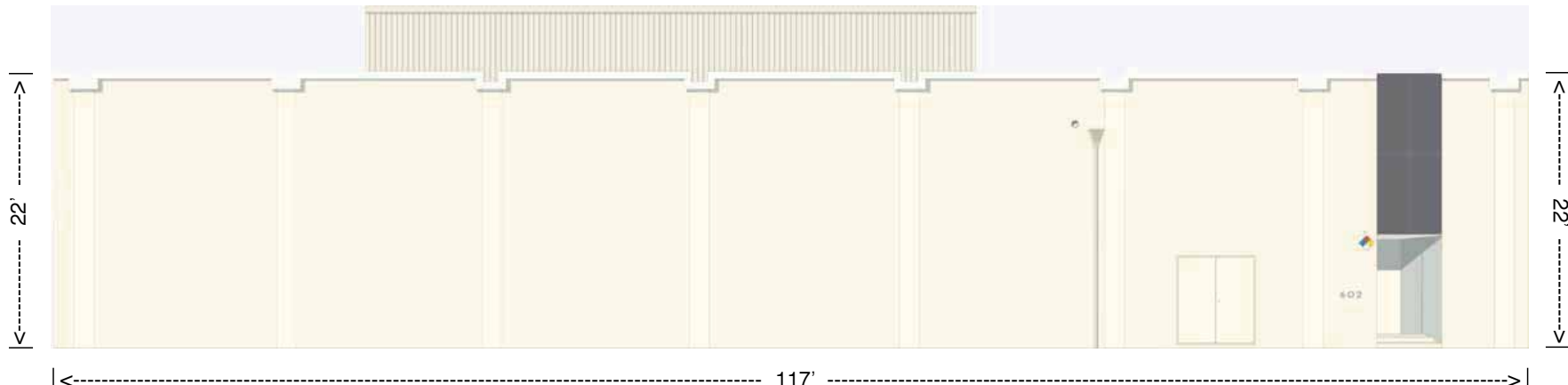
ACACIA AVENUE ELEVATION
