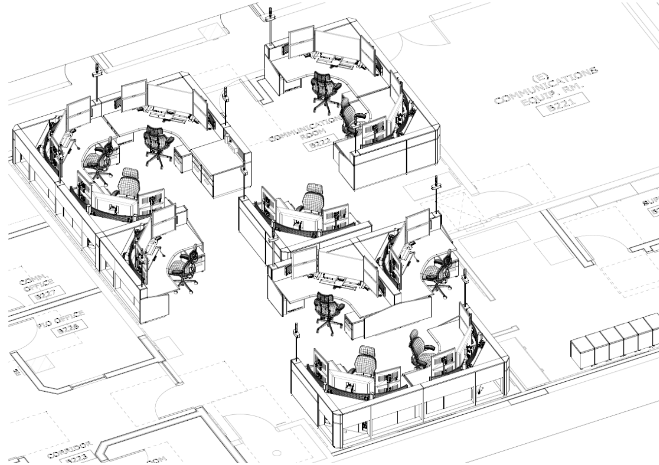
Expanded communications center layout
