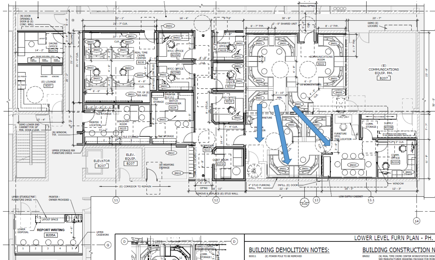
New communications center and lower level layout
