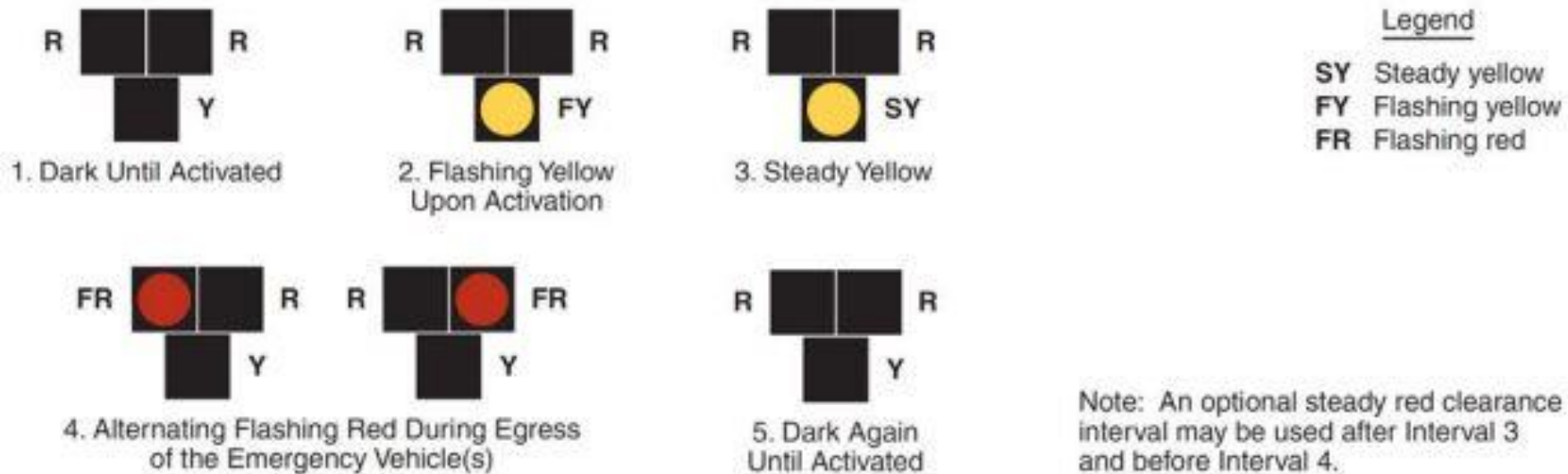
Figure 4G-1. Sequence for an Emergency-Vehicle Hybrid Beacon
