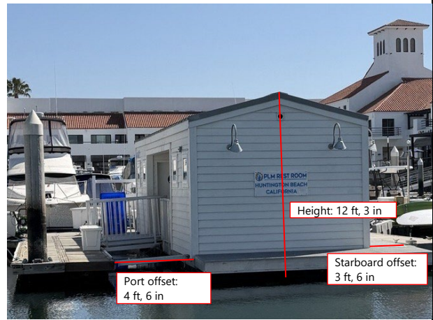
Photograph 6 Stern of Floating Restroom
