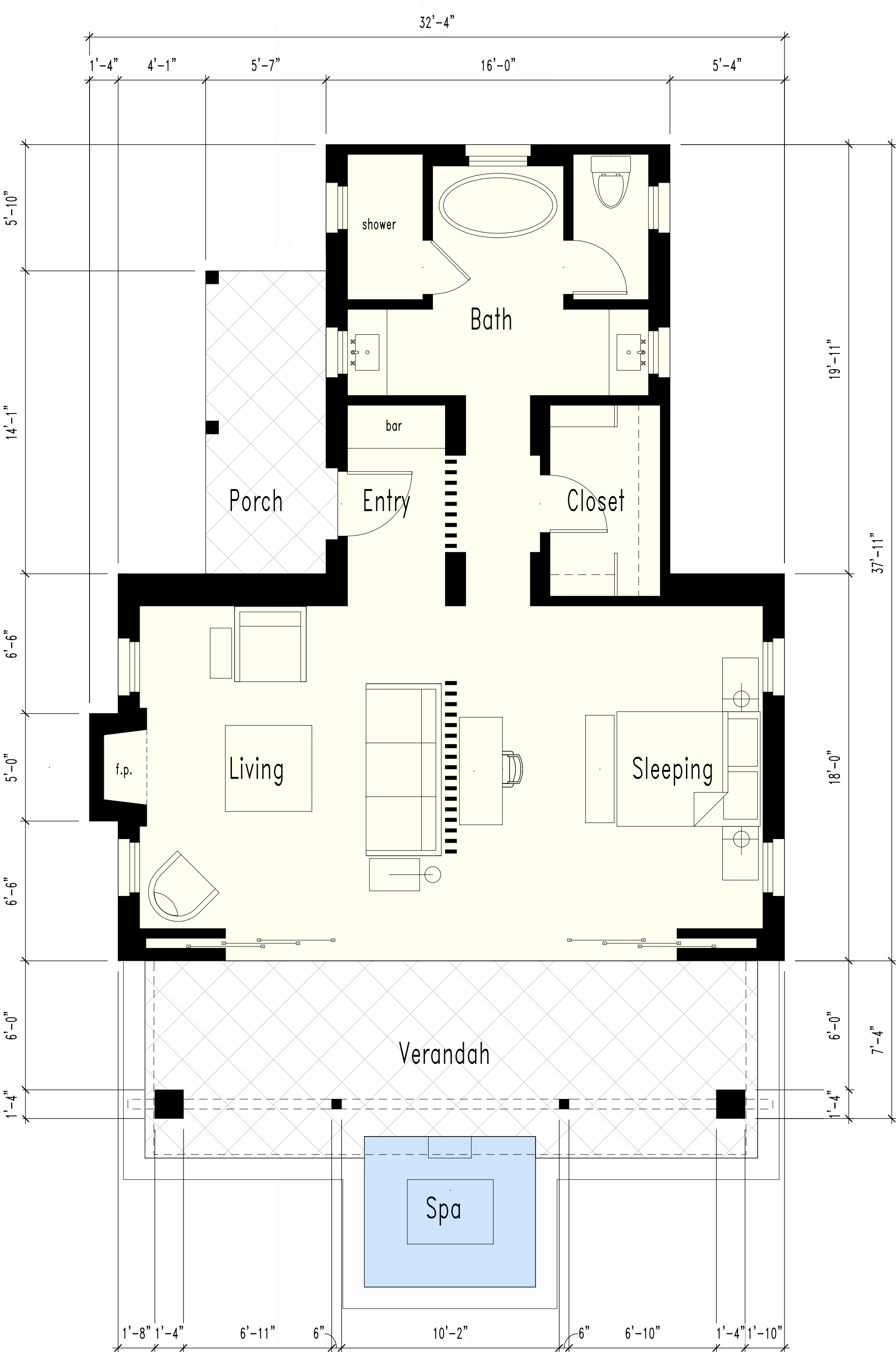
FLOOR PLAN
