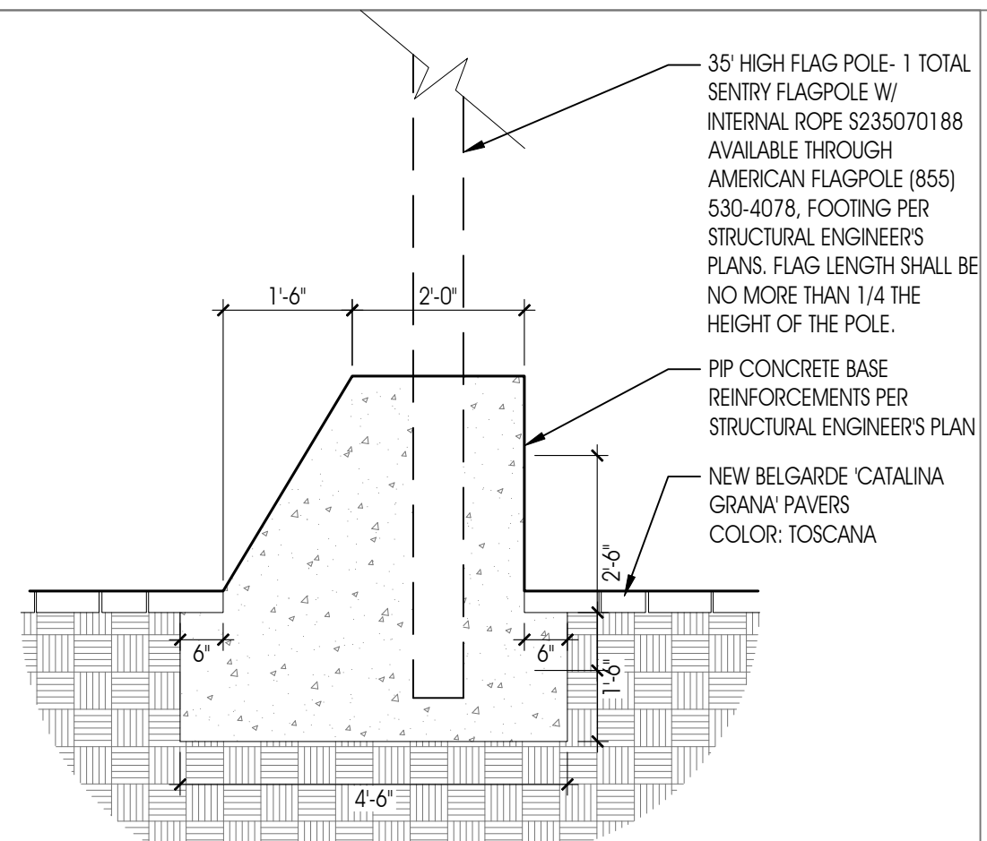
FLAGPOLE BASE
