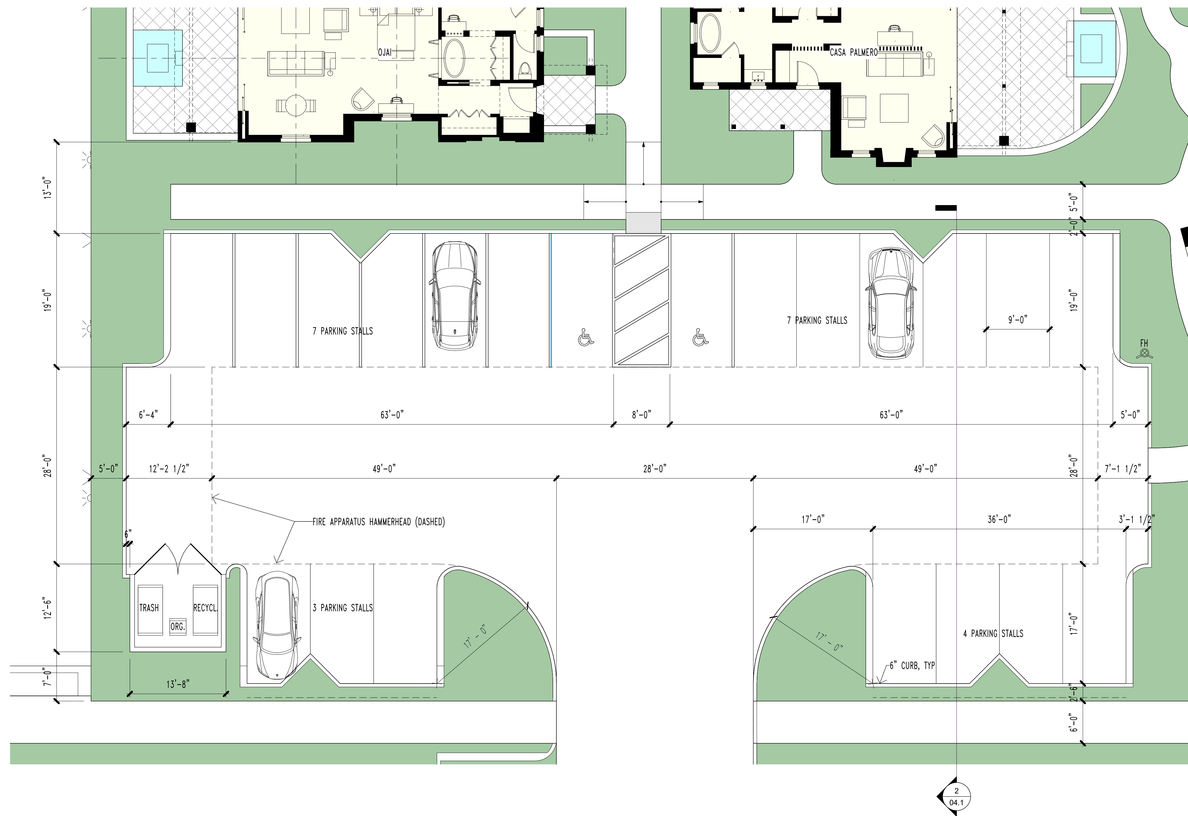
Enlarged Bungalow Parking Plan & Section 1/8" = 1'-0"
