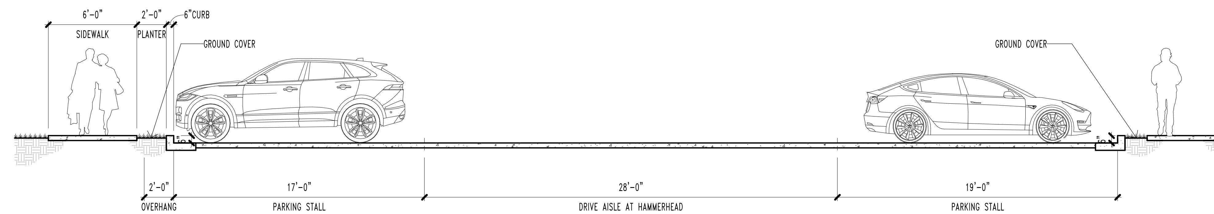
Section at Bungalow Parking 1/4" = 1'-0"
