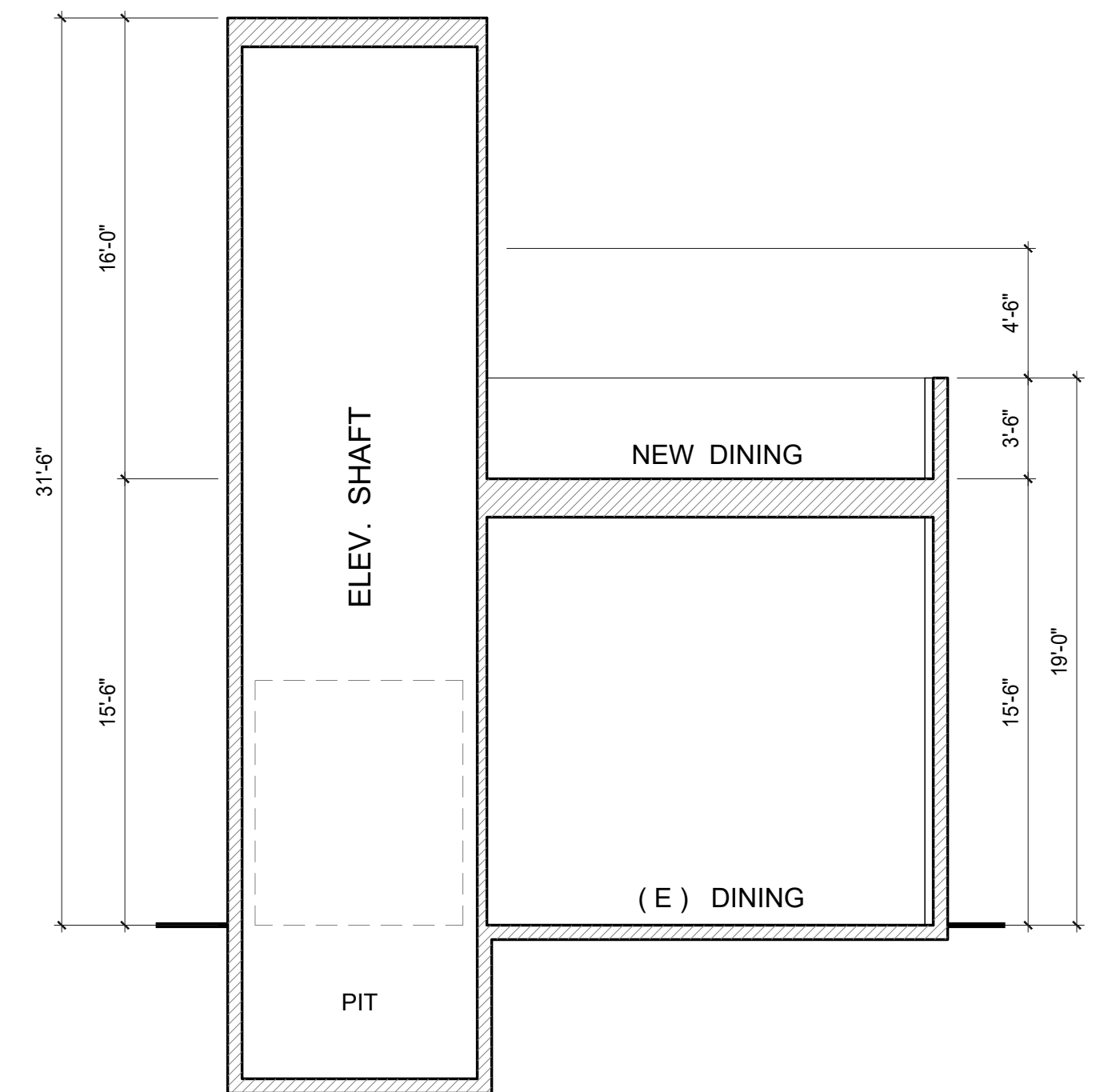
BUILDING SECTION
