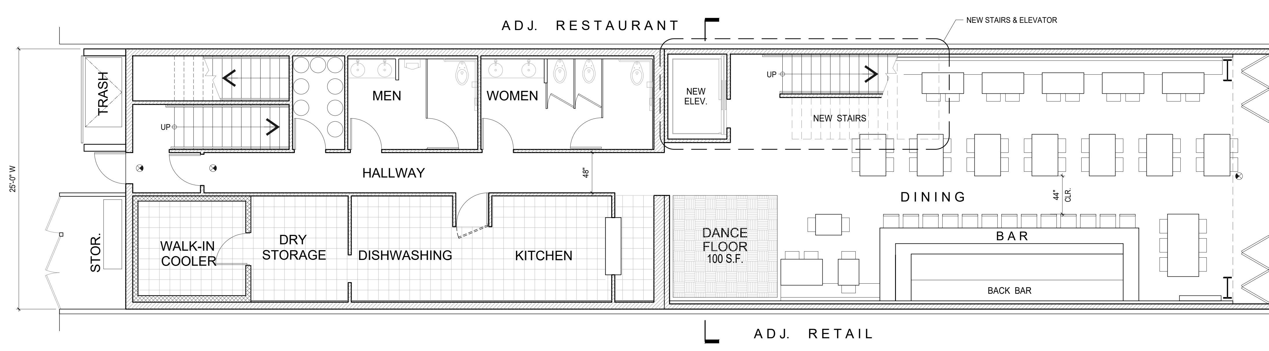
EXISTING GROUND FLOOR OCCUPANCY : 160 PERSONS
