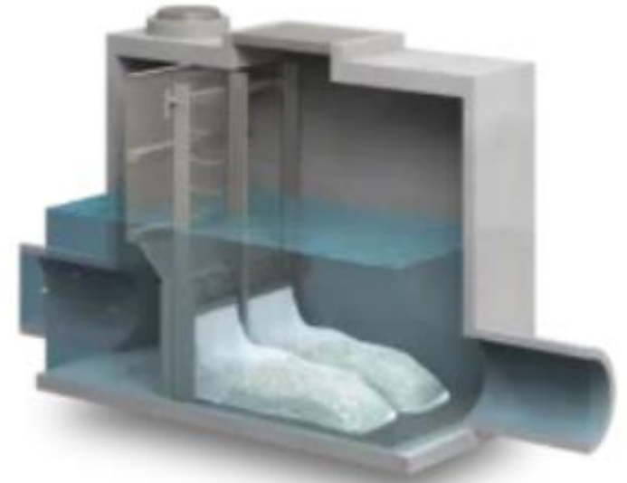
Inline TrashTrap
