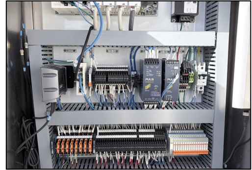
PLC Utility Station
