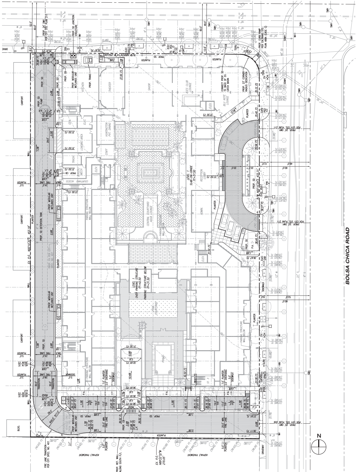
Exhibit 4.1: Grading Plan
