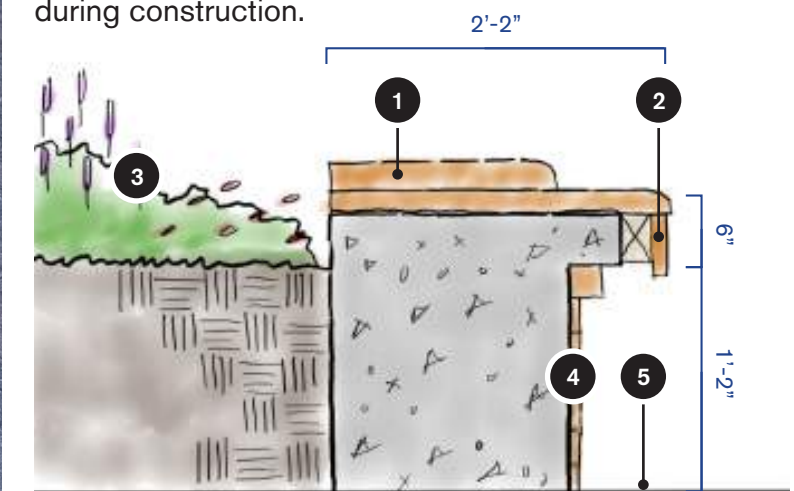
Existing Seatwall Section
