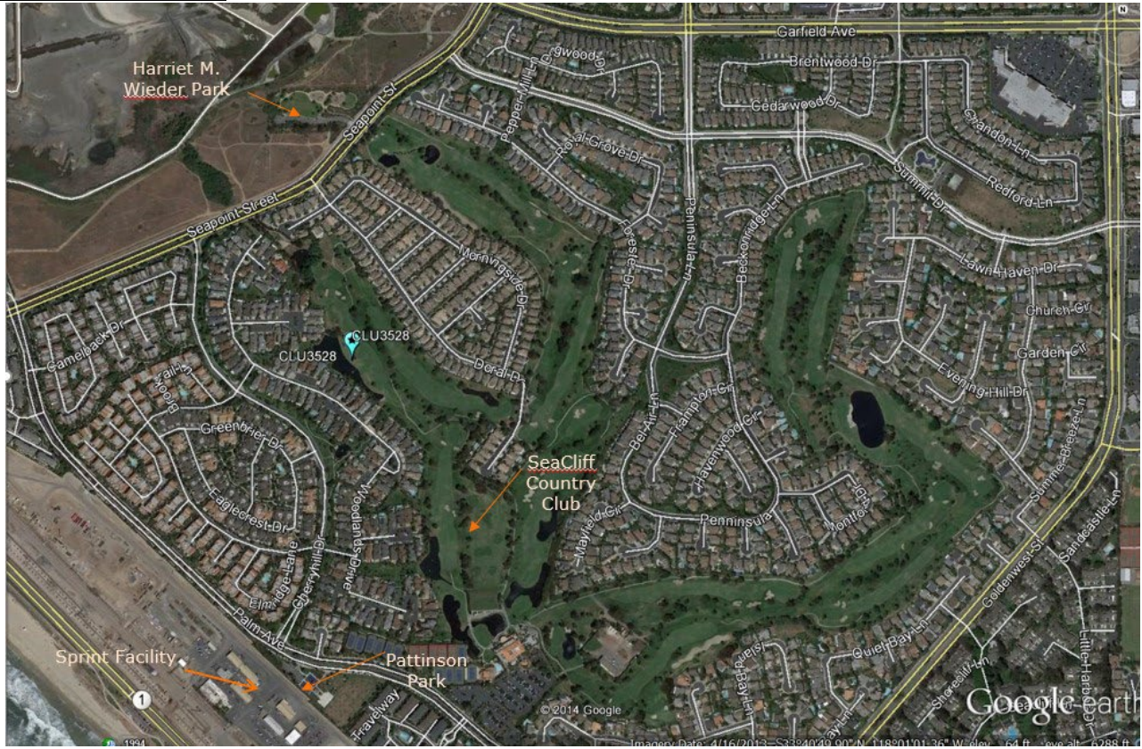
Exhausted Candidates
