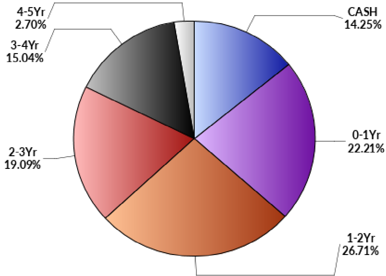
Maturity Distribution
