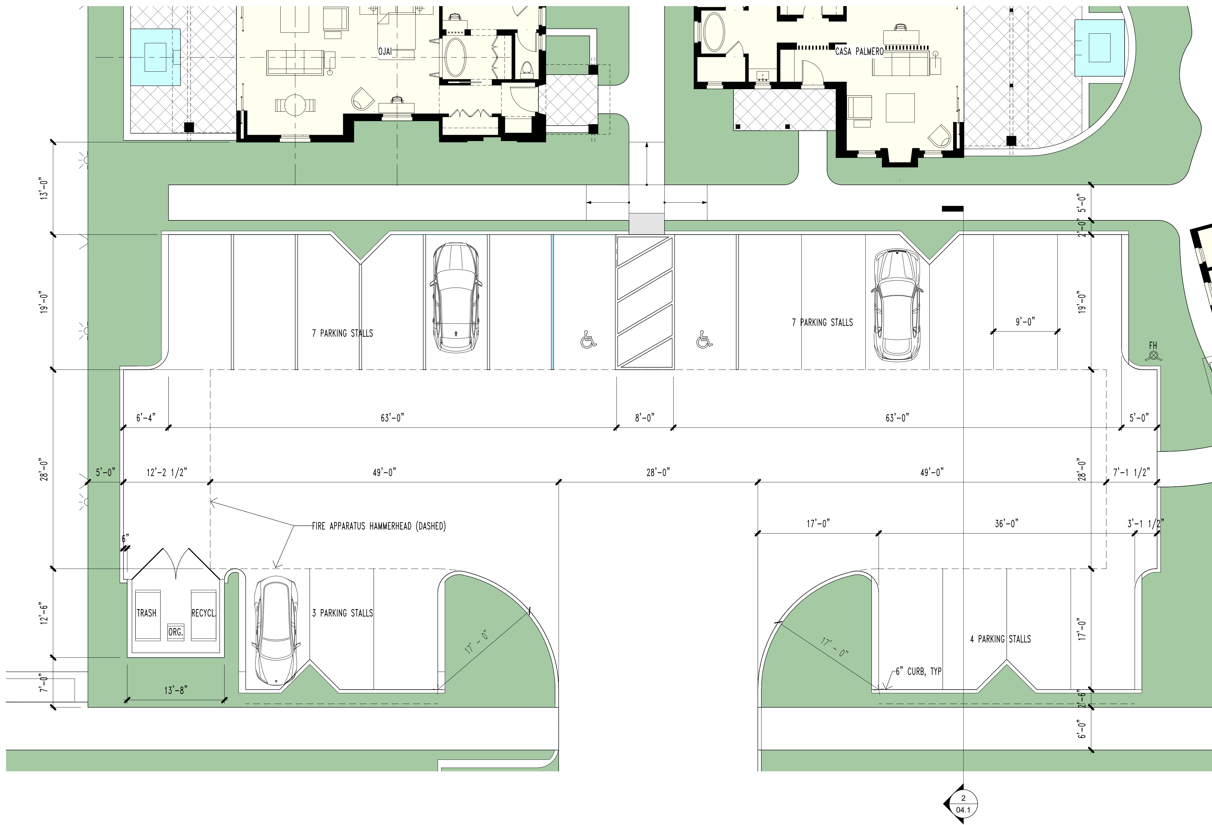
Enlarged Bungalow Parking Plan & Section 1/8" = 1'-0"
