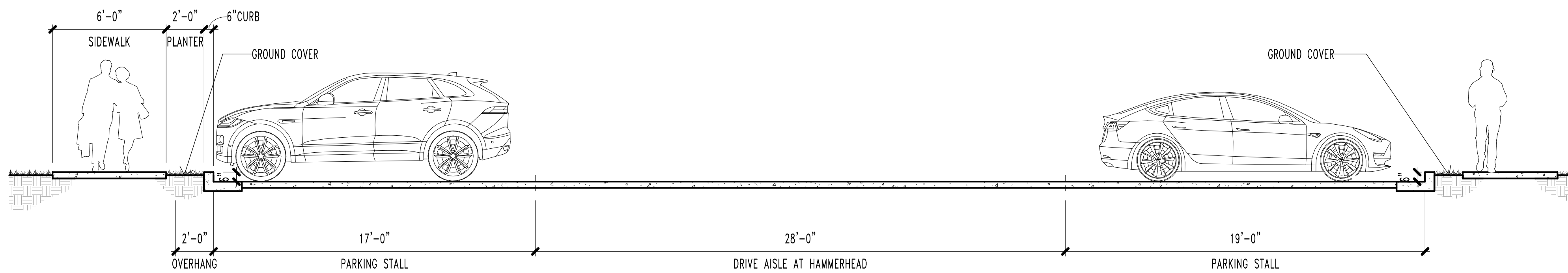
Section at Bungalow Parking 1/4" = 1'-0"
